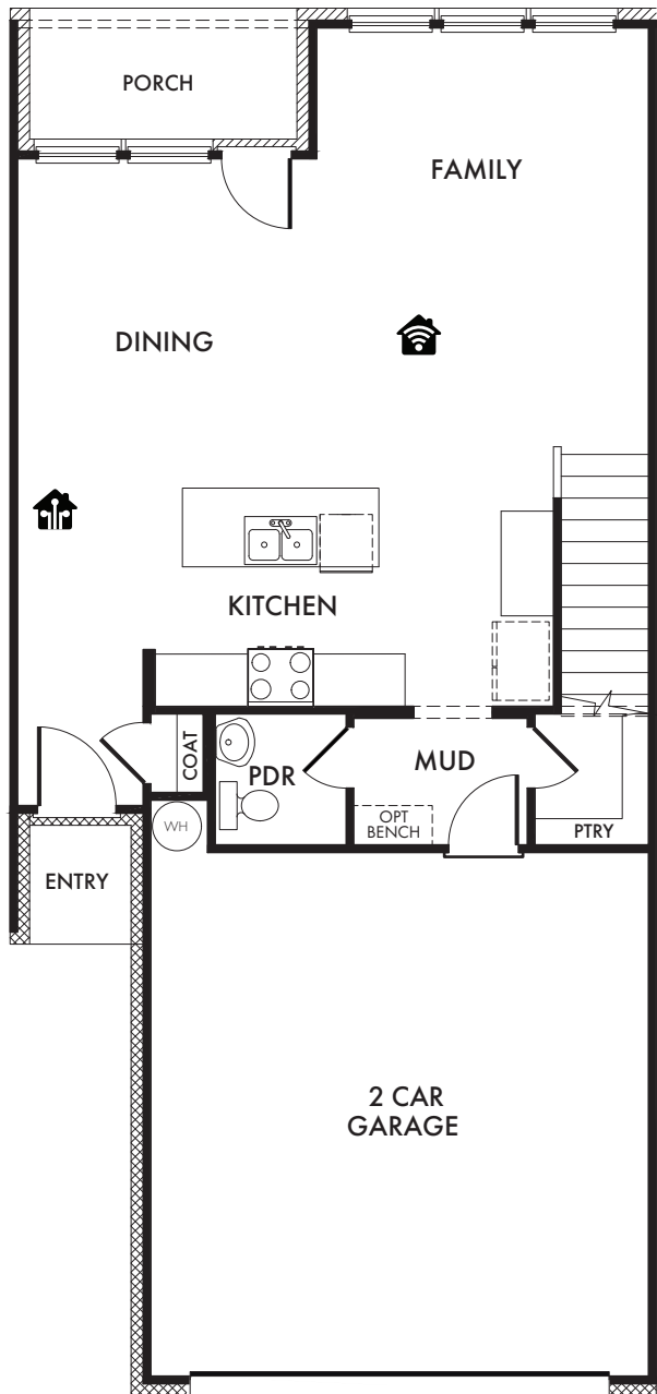
FIRST FLOOR
