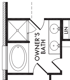
OPTIONAL OWNER'S BATH w/Full Wall OPT. #203
