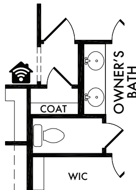
OPTIONAL OWNER'S BATH w/Double Sink Vanity Included Standard OPT. #206
