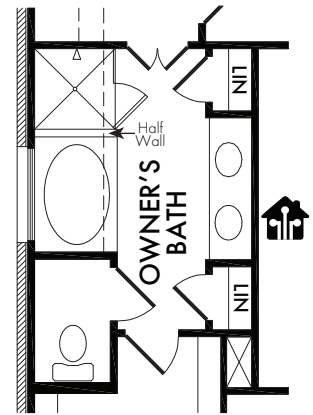
OPTIONAL OWNER'S BATH w/Half Wall OPT. #202
